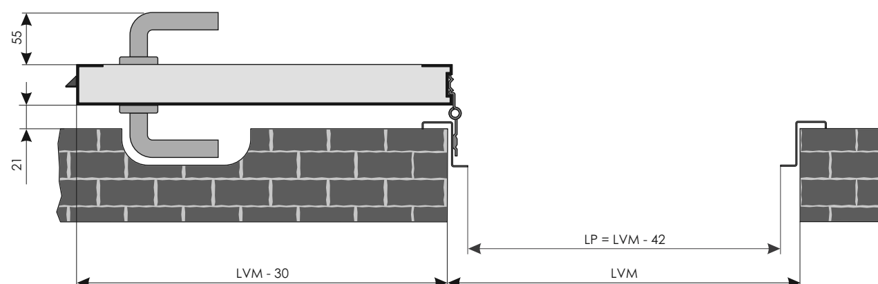
INGOMBRI PORTA CON APERTURA A 180° OPENING OVERALL DIMENSIONS WITH A 180° OPENING ANGLE
